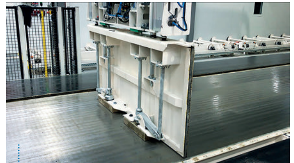
Fig. 6: The Aircrete Movable Mould Door in action: an automated door manipulator picks the movable door out of the door carrier and places it on the desired position.
