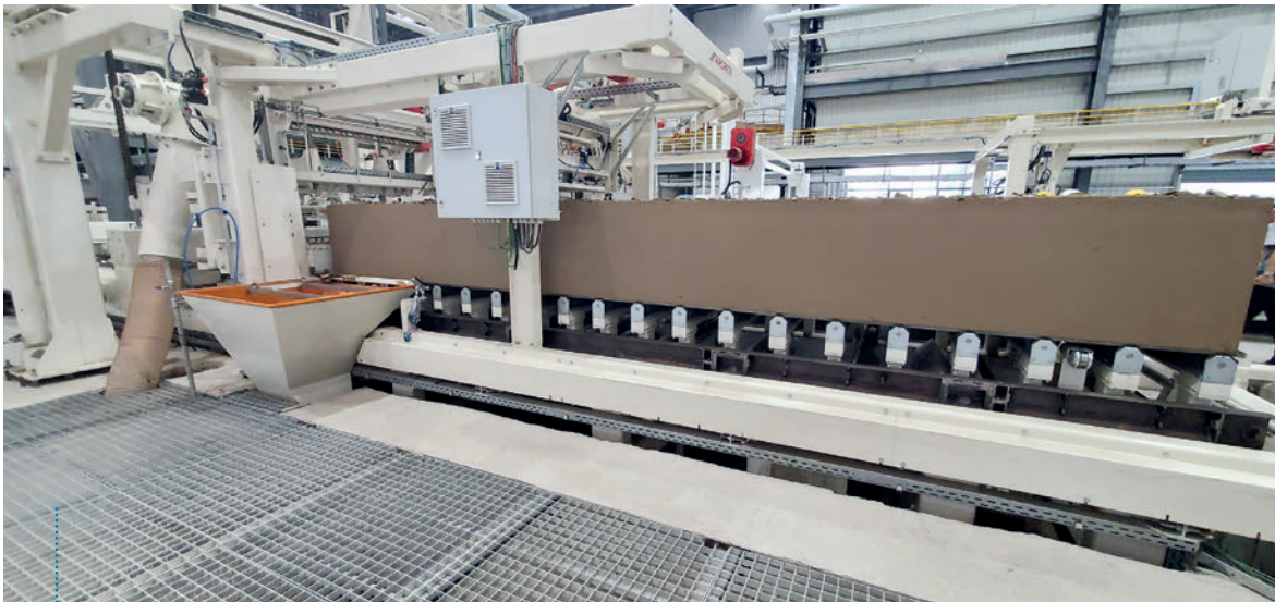
Fig. 7: In all Aircrete plants, the cake remains horizontal from casting, rising, cutting till unloading, and no separating nor green cake tilting machines are needed.
