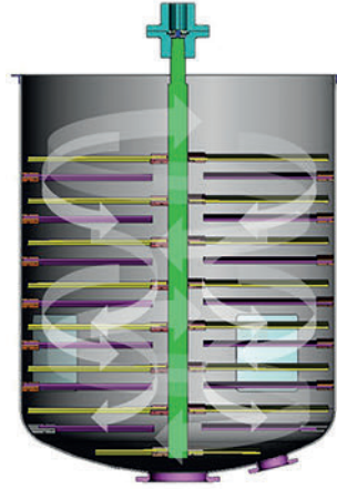
Fig. 3: The Aircrete low-speed mixer, with multiple paddles, ensures a better homogeneous mix.
